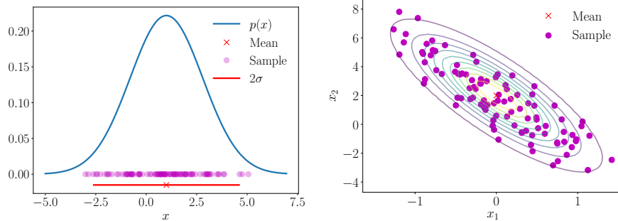
(a) Univariate (one-dimensional) Gaussian; The red cross shows the mean and the red line shows the extent of the variance. (b) Multivariate (two-dimensional) Gaussian, viewed from top. The red cross shows the mean and the colored lines show the contour lines of the density.
